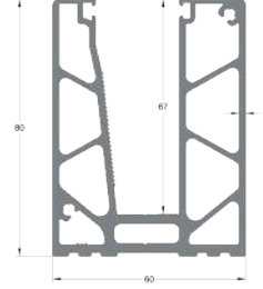
Tek Parça Baza 6 mt One Piece Base 6 m
